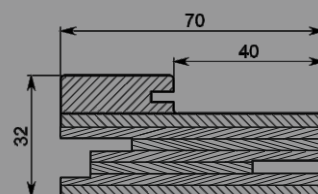
ADJUSTABLE DOOR FRAME (plywood + MDF) 70x32x2070mm 100x32x2070mm
