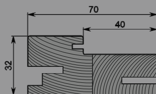
ADJUSTABLE DOOR FRAME (wood) 70x32x2070mm 100x32x2070mm
