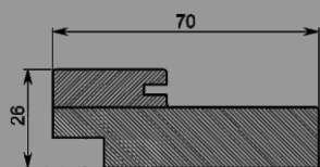
DOOR FRAME (with seal) 70x26x2070mm
