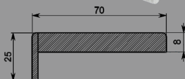
ADJUSTABLE ARCHITRAVE (MDF) 70(17)x8x2150mm 100(17)x8x2150mm
