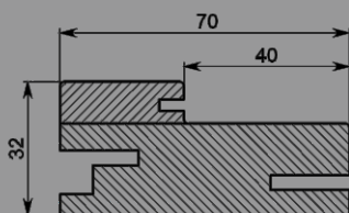
ADJUSTABLE DOOR FRAME (MDF) 70x32x2070mm 100x32x2070mm
